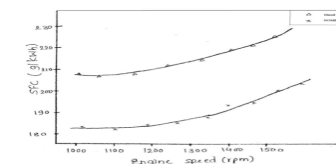
Figure 2: Specific fuel consumption (SFC) for Diesel Oil and NOME Biodiesel Blends
