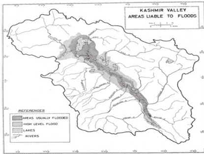
Figure 6: Flood affected region of the Jhelum river
