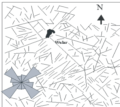
Figure 5: Drainage lineament map of the region around the Wular lake
