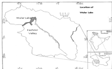
Figure 1: Location map of the Wular lake
