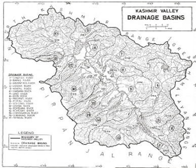
Figure 3: Main drainage of the Kashmir valley
