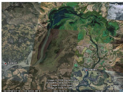
Figure 4: The bird's eye view of the Wular lake
