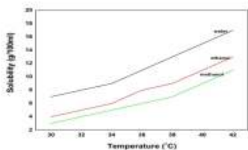
Figure 2: Solubility curve of PLT single crystal
